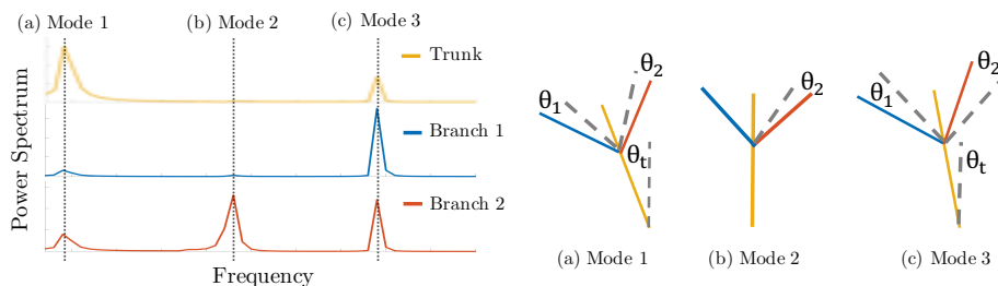
Fig. 6. Mode shapes. The left three curves show the power spectra of the trunk and the two branches. The three mode shapes extracted from vibration are shown on the right. total energy for every time-stepping update. If the system’s energy increases during an update, we rescale the kinetic and potential energy of each branch to ensure that the total energy of the system is constant. This makes our simulation robust and stable. See the supplementary material for the detailed derivation.
