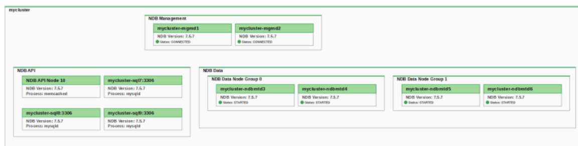
Figure 29.4 NDB Cluster Topology
