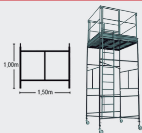
ANDAIME TUBULAR DE 1,0 x 1,5m
